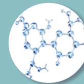
Tripeptide GHK
